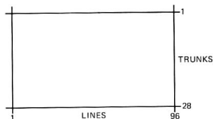
Fig. 3—One-stage network.
