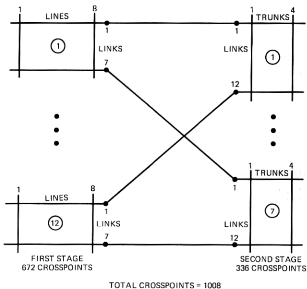
Fig. 4—Two-stage network.
